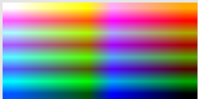
scaled
