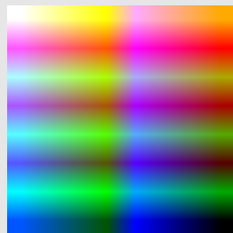
interpolated
