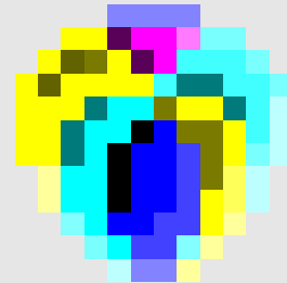
inverted
