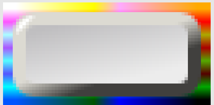
on Background
